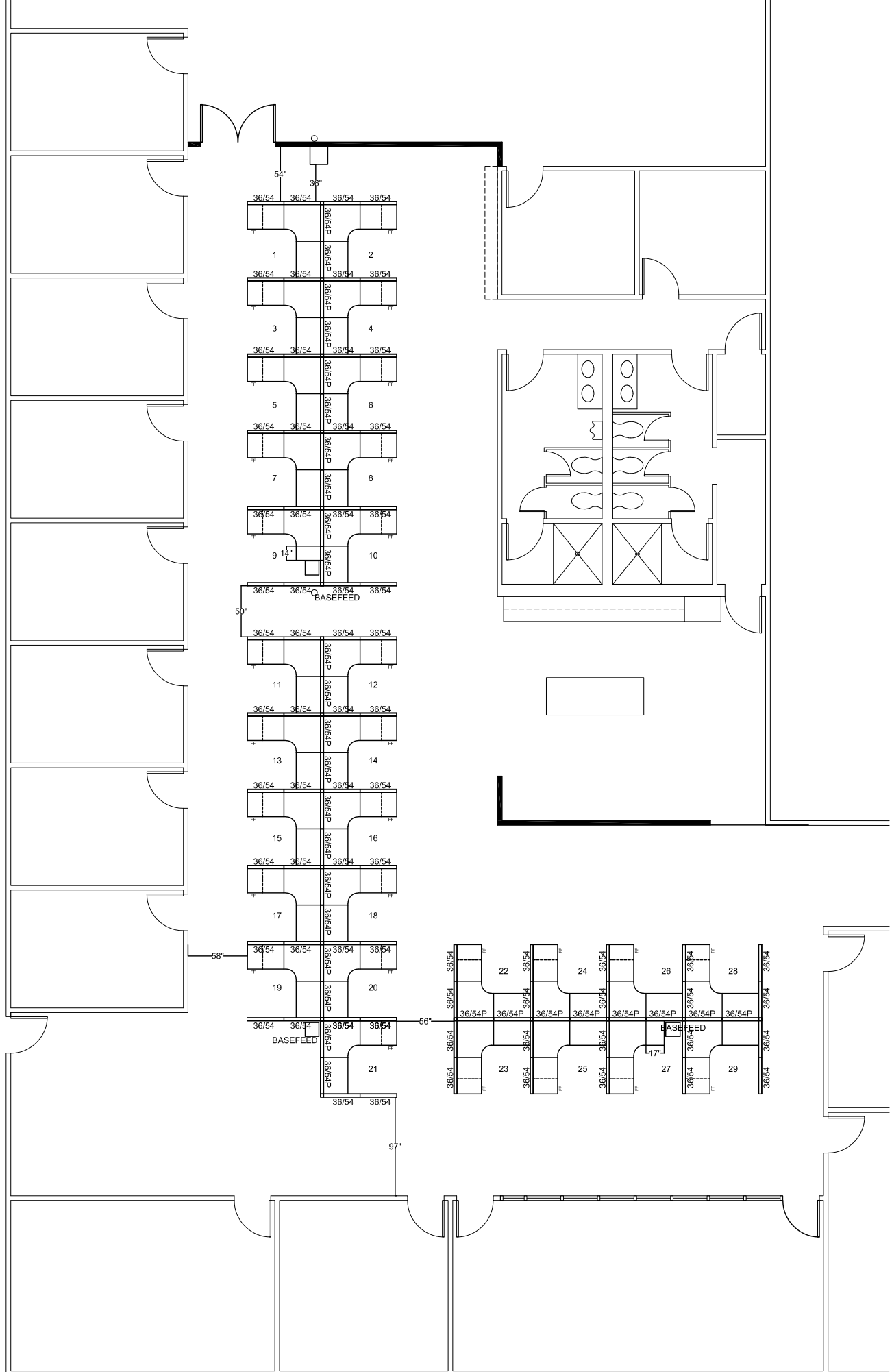
Furniture Layout - Richardson Location Scale: NTS
